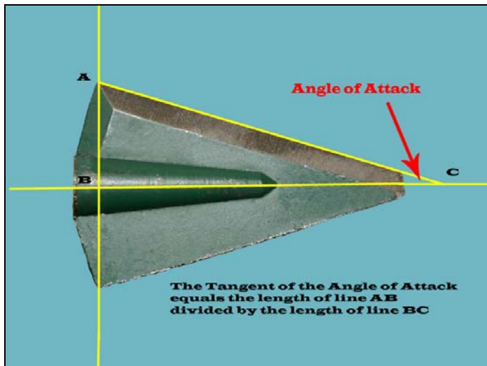
Angle of attack calculations for the 190 gr. Abowyer Custom.
