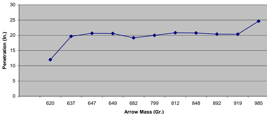
Graph 2 Extreme FOC's: Arrow Mass and Average Penetration All Shots; All Broadheads 2005 Asian Buffalo Testing N=39
